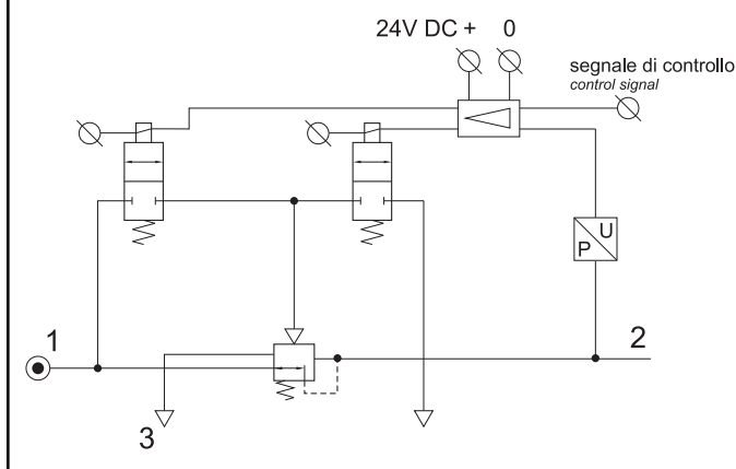
Schema pneumatico Pneumatic diagram
